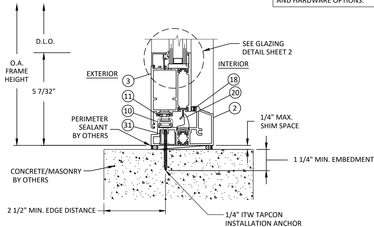
A 4 VERTICAL SECTION SILL - CONCRETE/MASONRY STANDARD SILL
