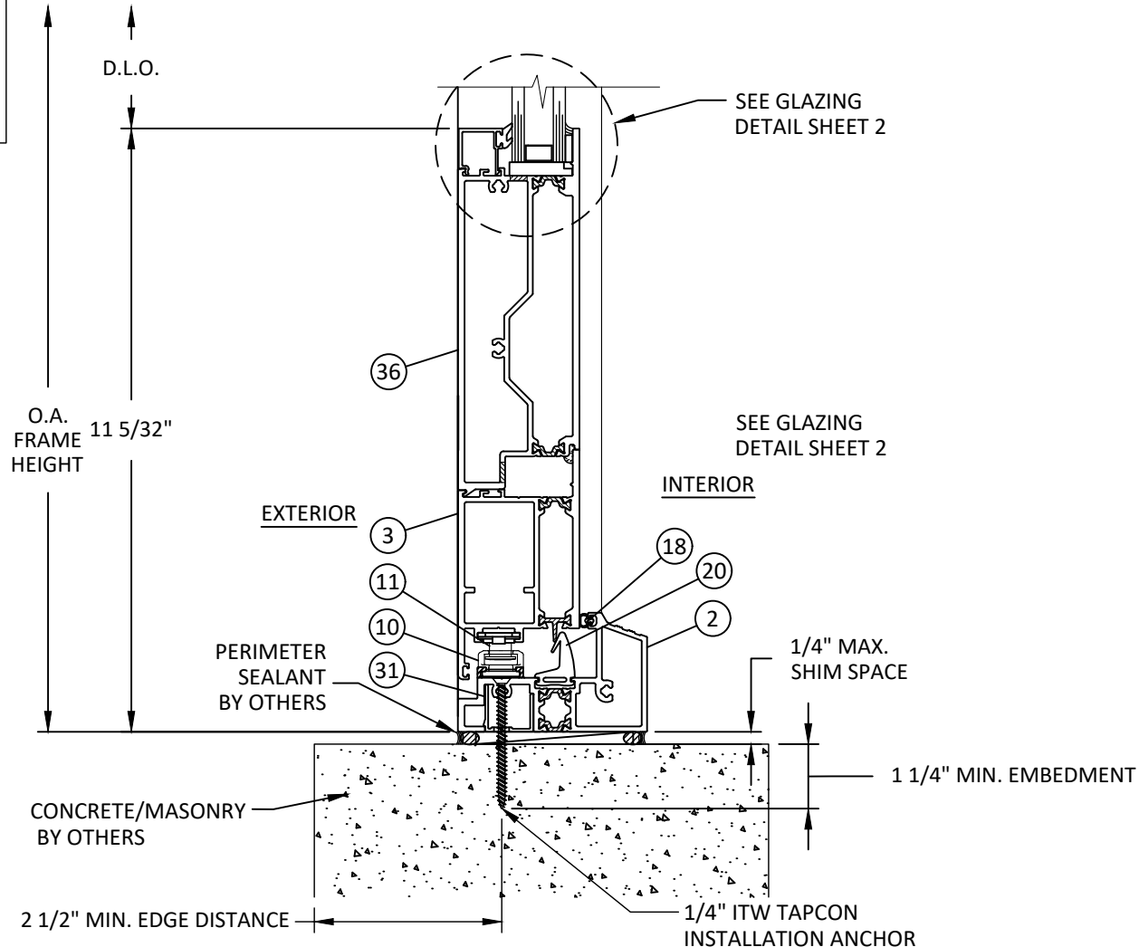
D 4 VERTICAL SECTION SILL - CONCRETE/MASONRY 10" BOTTOM RAIL W/ STANDARD SILL
