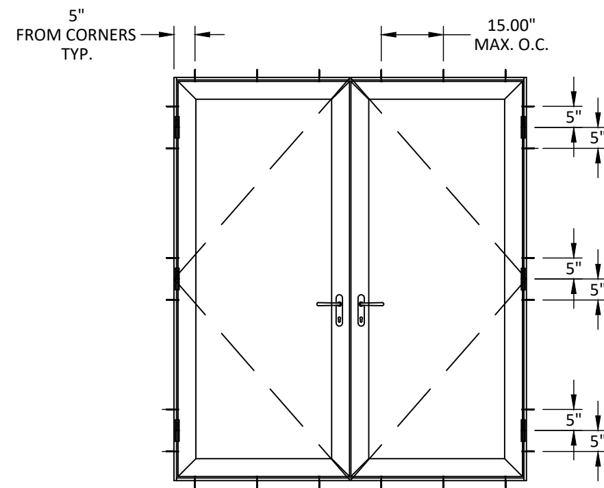
ANCHOR LAYOUT TYPICAL
