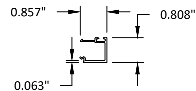
5 GLASS STOP
