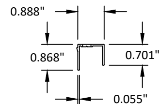
31 ANCHOR FILLER
