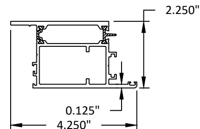
5 GLASS STOP
