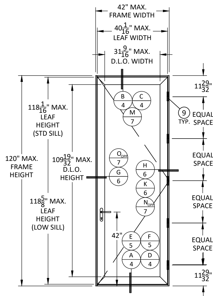
ELEVATION STANDARD SILL ONLY OR LOW PROFILE SILL
