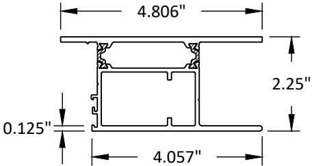
35 BOTTOM RAIL (LOW SILL)
