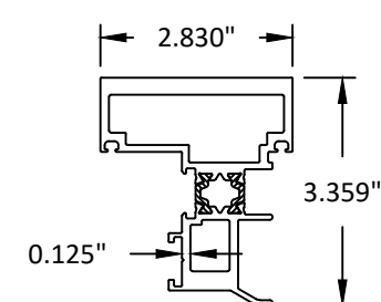
8 CORNER KEY
