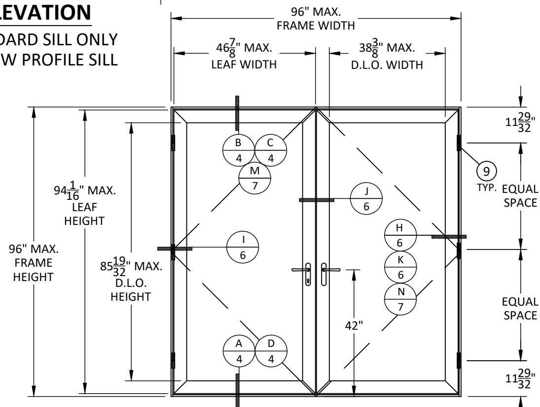
ELEVATION STANDARD SILL ONLY
