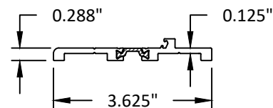
33 LOW PROFILE SILL
