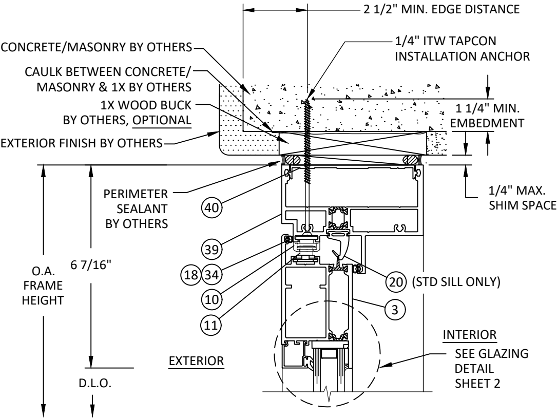
M 7 VERTICAL SECTION HEAD - CONCRETE/MASONRY YWW FRAME
