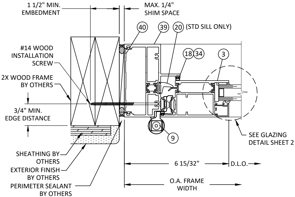
N 7 HORIZONTAL SECTION HINGE JAMB - WOOD FRAME YWW FRAME
