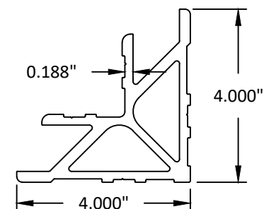
33 LOW PROFILE SILL
