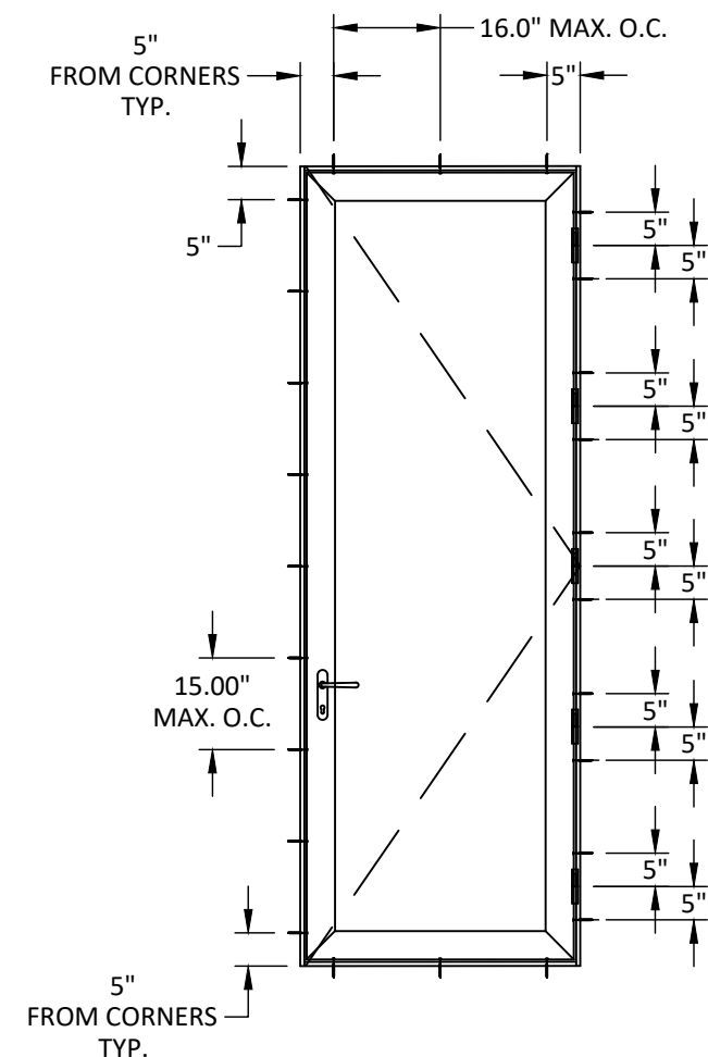
ANCHOR LAYOUT TYPICAL
