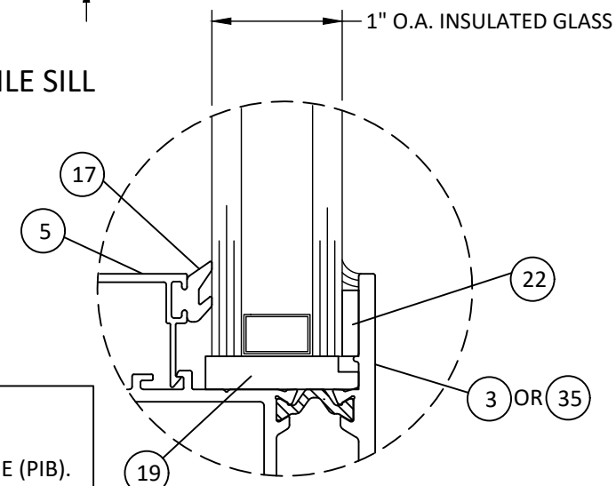
GLAZING DETAIL
