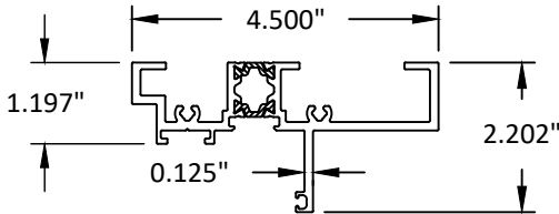
37 4 1/2" FRAME HEAD/JAMB
