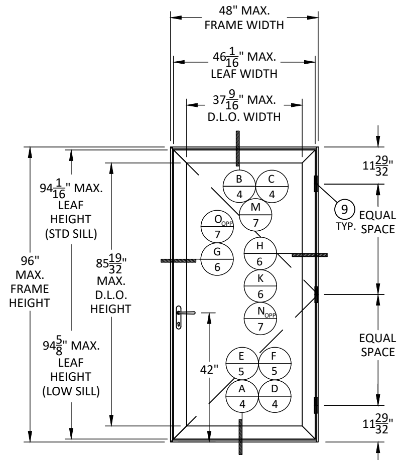
ELEVATION STANDARD OR LOW PROFILE SILL
