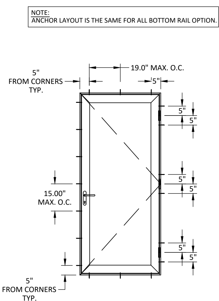
ANCHOR LAYOUT TYPICAL
